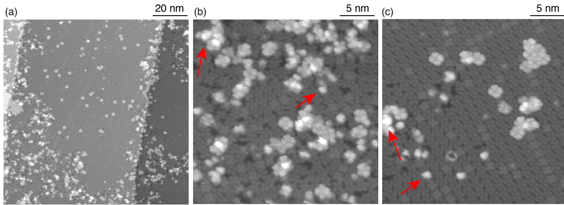
FIG. S3. STM images of a sample with a ratio between Tb and 2H-Pc molecules exceeding 0.5 and a 2H-Pc coverage lower than 2 ML (1.2 ML 2H-Pc/Ag(111) + 0.8 ML Tb). (a) Large scale image. (b), (c) zoom on different regions showing TbPc 2 molecules (gray) embedded in the 2H-Pc layer (dark gray) and Tb clusters (white dots). Red arrows point to some clusters. ( V_t = -2.0 V, I_t = 50 pA, T = 78 K).
