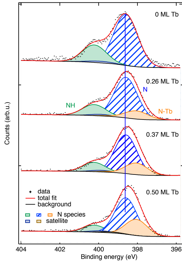
FIG. S2. N1s XPS spectra and corresponding fit for 1.9 ML pristine 2H-Pc molecules (upper panel) and after successive deposition of Tb. The amount of Tb is determined from the fit of the spectra including the different components.
