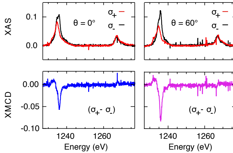
FIG. S1. XAS and XMCD spectra of 0.6 ML Tb atoms deposited directly on Ag(111) at RT. The spectral features of XAS and the magnitude of XMCD significantly differ from those of on-surface synthesized as well as ex-vacuo synthesized TbPc 2 , and point to an in-plane easy axis ( \mu_0 H = 6.8 T, T = 3 K).
