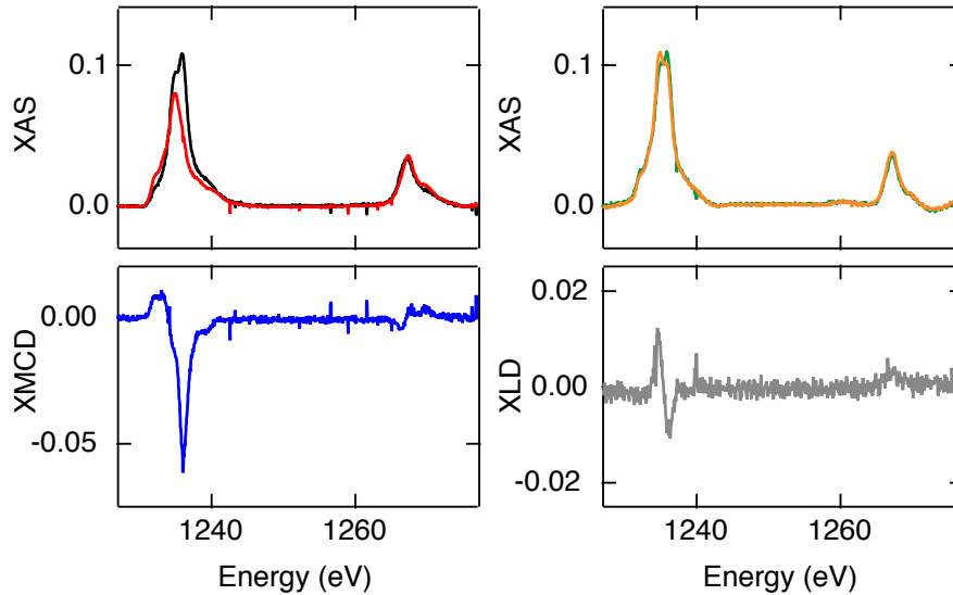
FIG. S4. (left) Normal incidence XAS and XMCD spectra and (right) grazing incidence XAS and XLD spectra of a sample with a ratio between Tb and 2H-Pc molecules exceeding 0.5 and a 2H-Pc coverage lower than 2 ML (1.4 ML 2H-Pc/Ag(111) + 2.0 ML Tb). The XMCD is strongly reduced with respect to the one shown in Fig. 1 in the main text for TbPc 2 molecules. In addition, the XLD is reduced and reversed in sign (left: \mu_0 H = 6.8 T, right: \mu_0 H = 0.05 T; T = 3 K).
